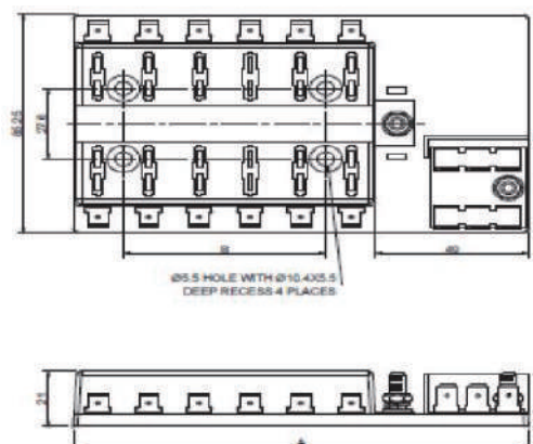
12 Way Fuse Holder Terminal C001-028-014612
